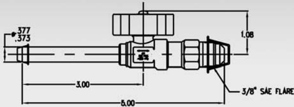
586WAR-6M6FL (3/8") Charging and Suction
