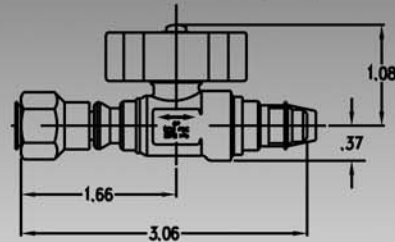
586WAR-6SW6FL (3/8") Retro Charging and Suction
