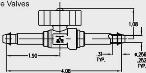
586WAR-4ST (1/4") & 586WAR-6ST (3/8") Line Valves
