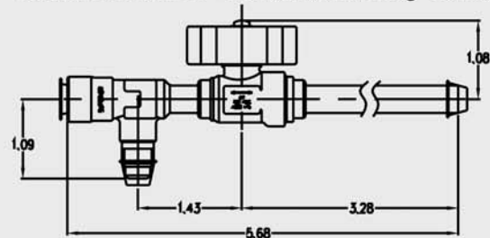
586WASR-6M2FP Control Monitoring Transducer
