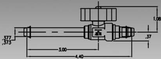
586WASR-6M (1/4") Access Shut-Off
