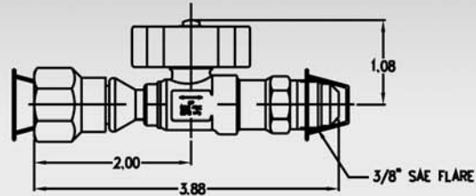
586WAR-6SW6FL (3/8") Retro Charging and Suction
