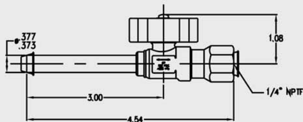
586WAR-6M4FP Pressure Control
